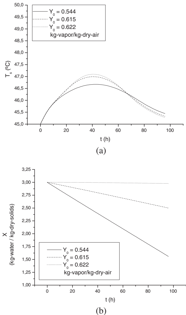
Fig. 4. Effect of inlet air moisture content on solid-phase variables: (a) T_s ( z/L = 0.925 ; r/R = 0.05 ); (b) X ( z/L = 0.075 ; r/R = 0.05 ).
