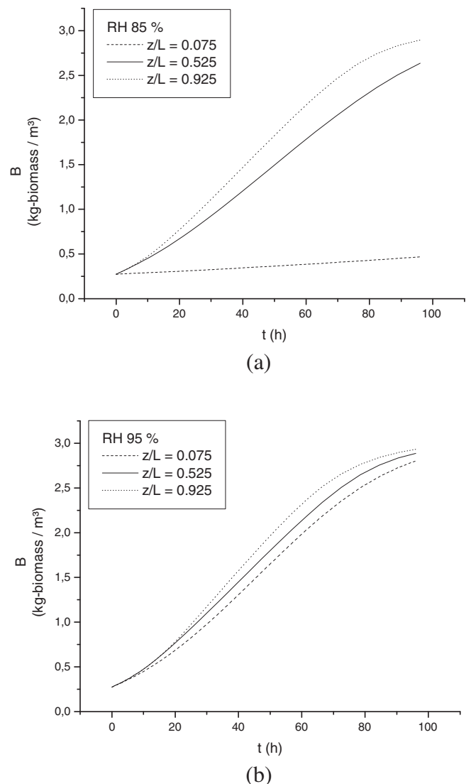
Fig. 5. Biomass concentration time-profiles: (a) for inlet air with RH 85%; (b) for inlet air with RH 95%.
